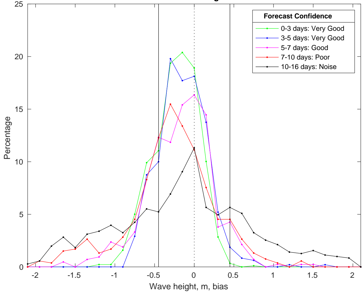
NDBC 46028 vs GFSWaves Bias Histogram: 20-Jan-2025
