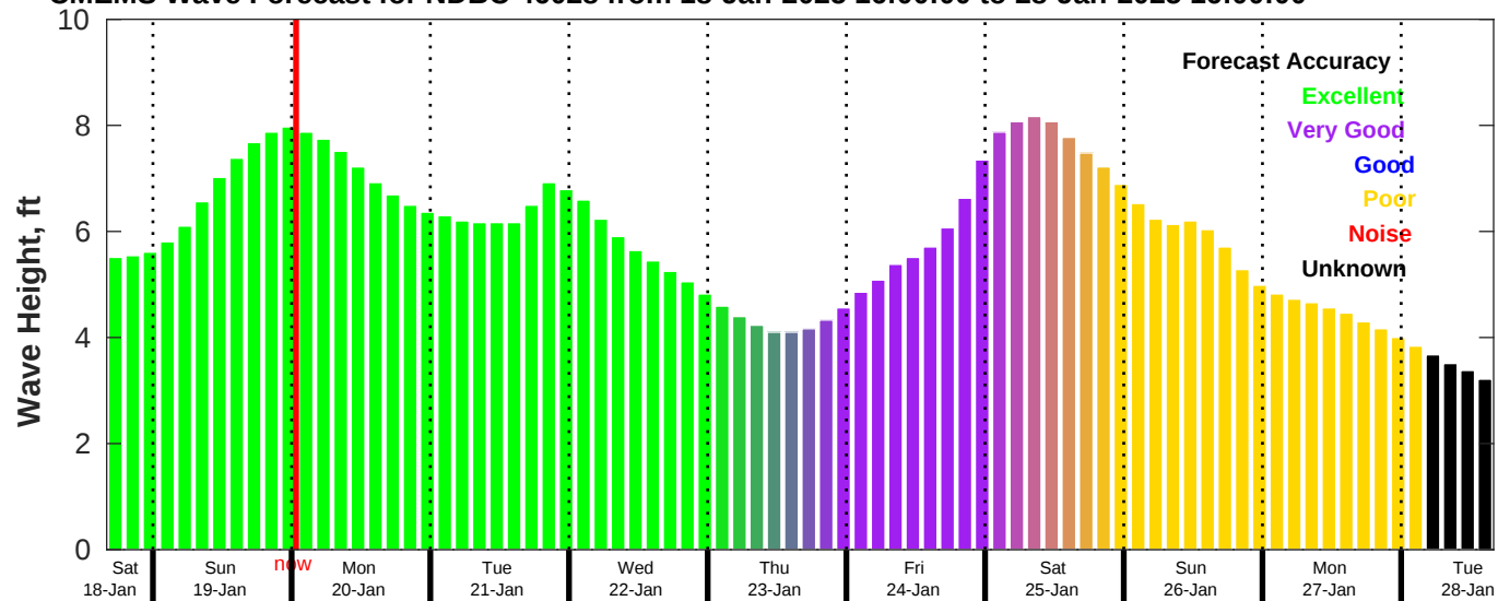
CMEMS Wave Forecast for NDBC 46028 from 18-Jan-2025 16:00:00 to 28-Jan-2025 16:00:00
