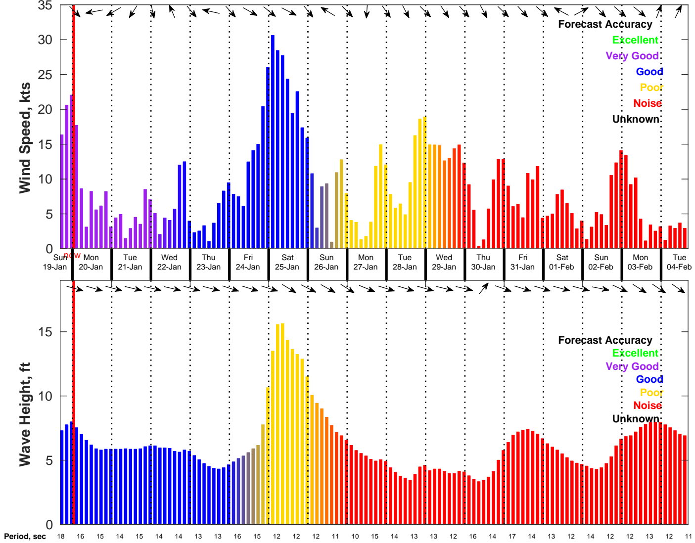
Wind & Wave Forecast for NDBC 46028 from 19-Jan-2025 16:00:00 to 04-Feb-2025 16:00:00
