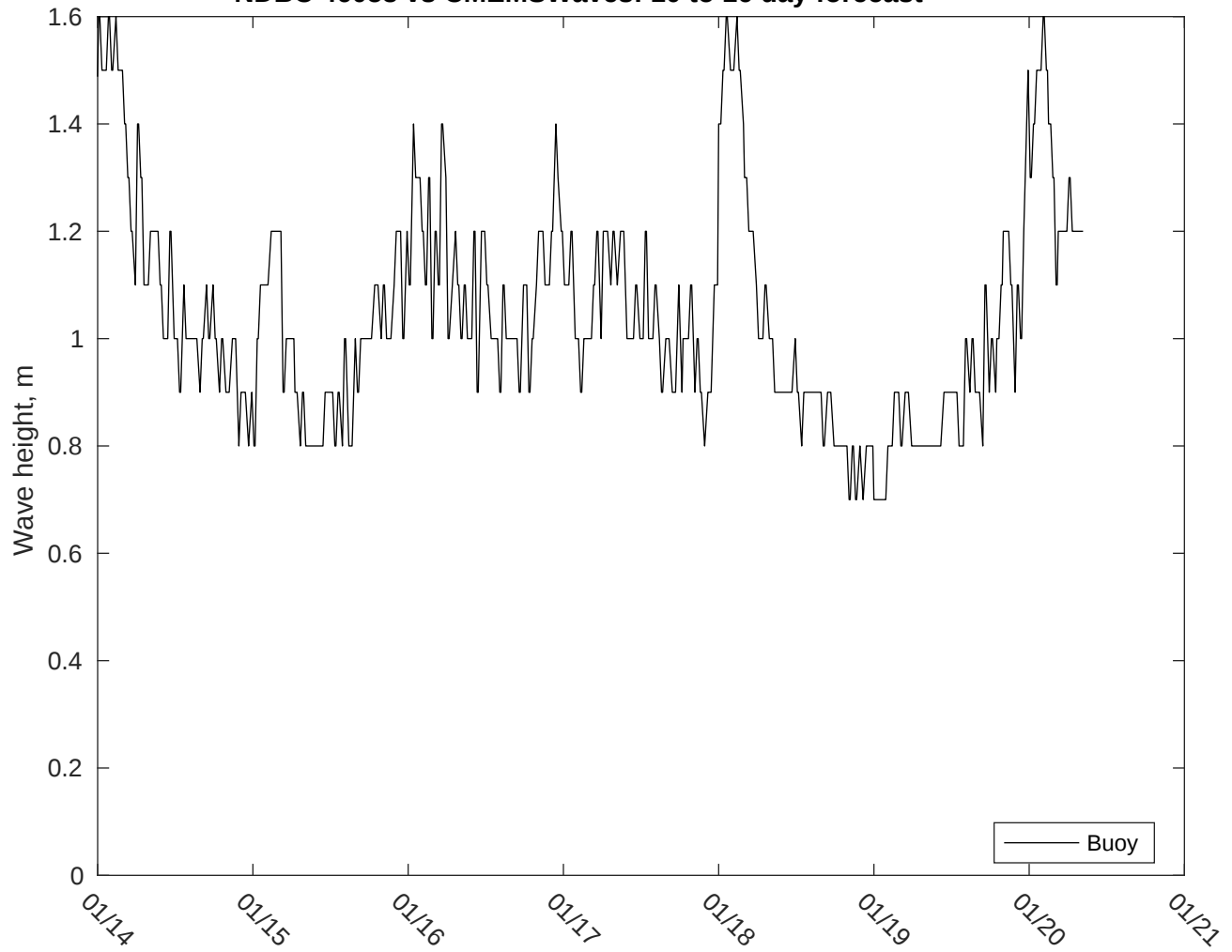
NDBC 46053 vs CMEMSWaves: 10 to 16 day forecast
