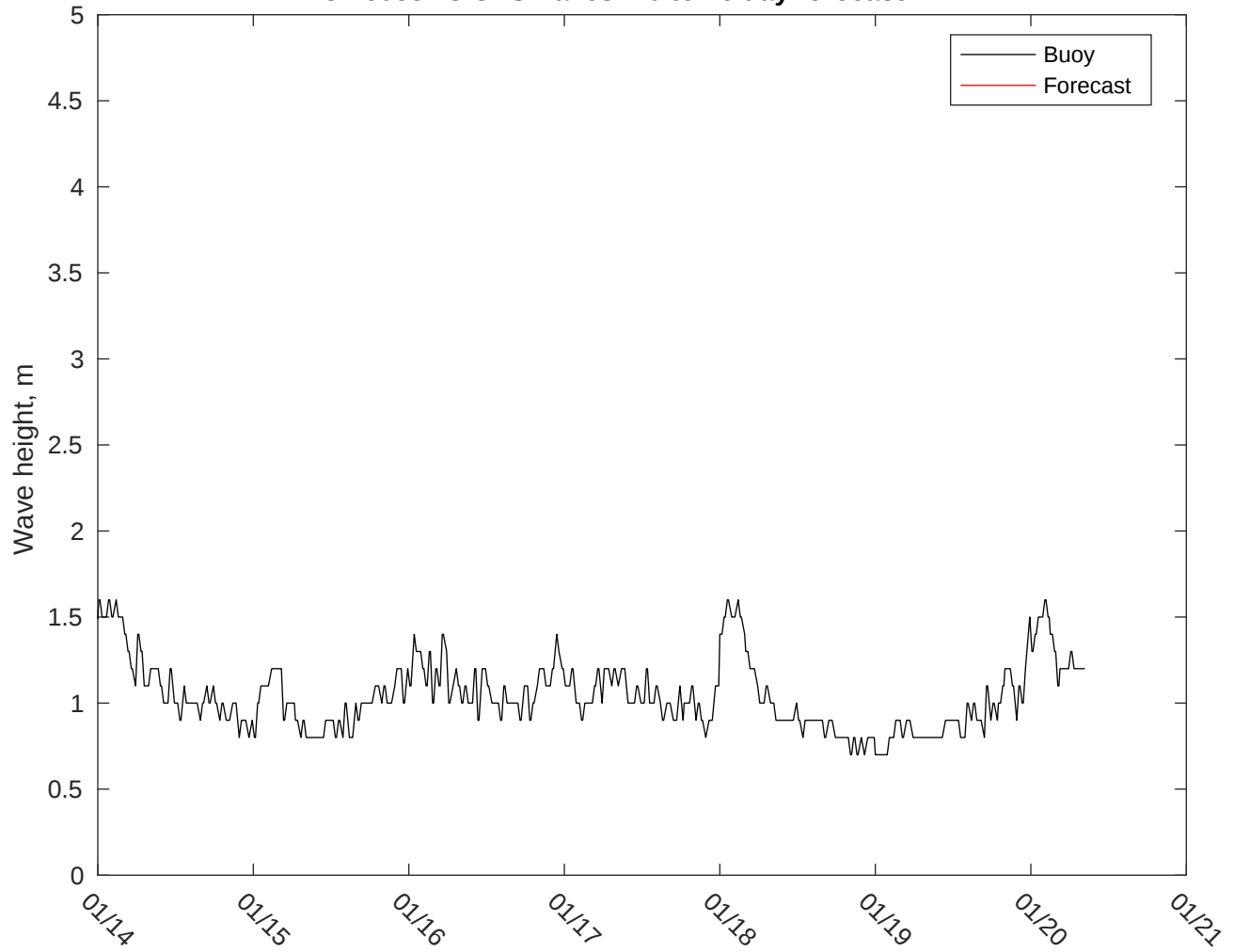
NDBC 46053 vs GFSWaves: 10 to 16 day forecast
