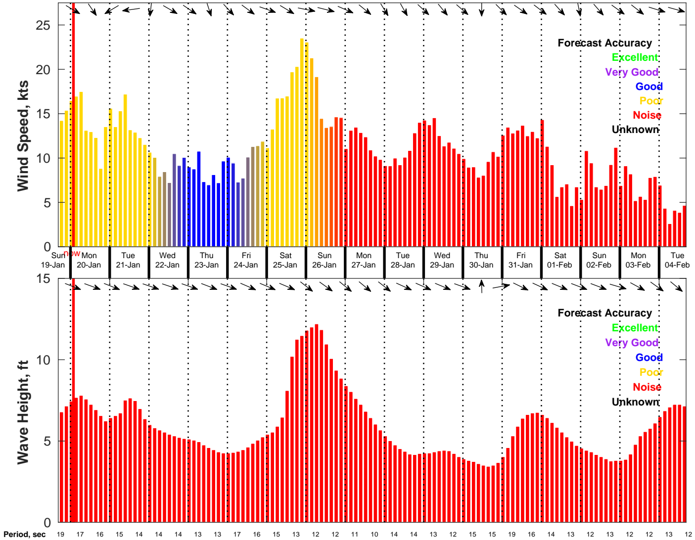
Wind & Wave Forecast for NDBC 46053 from 19-Jan-2025 17:00:00 to 04-Feb-2025 17:00:00
