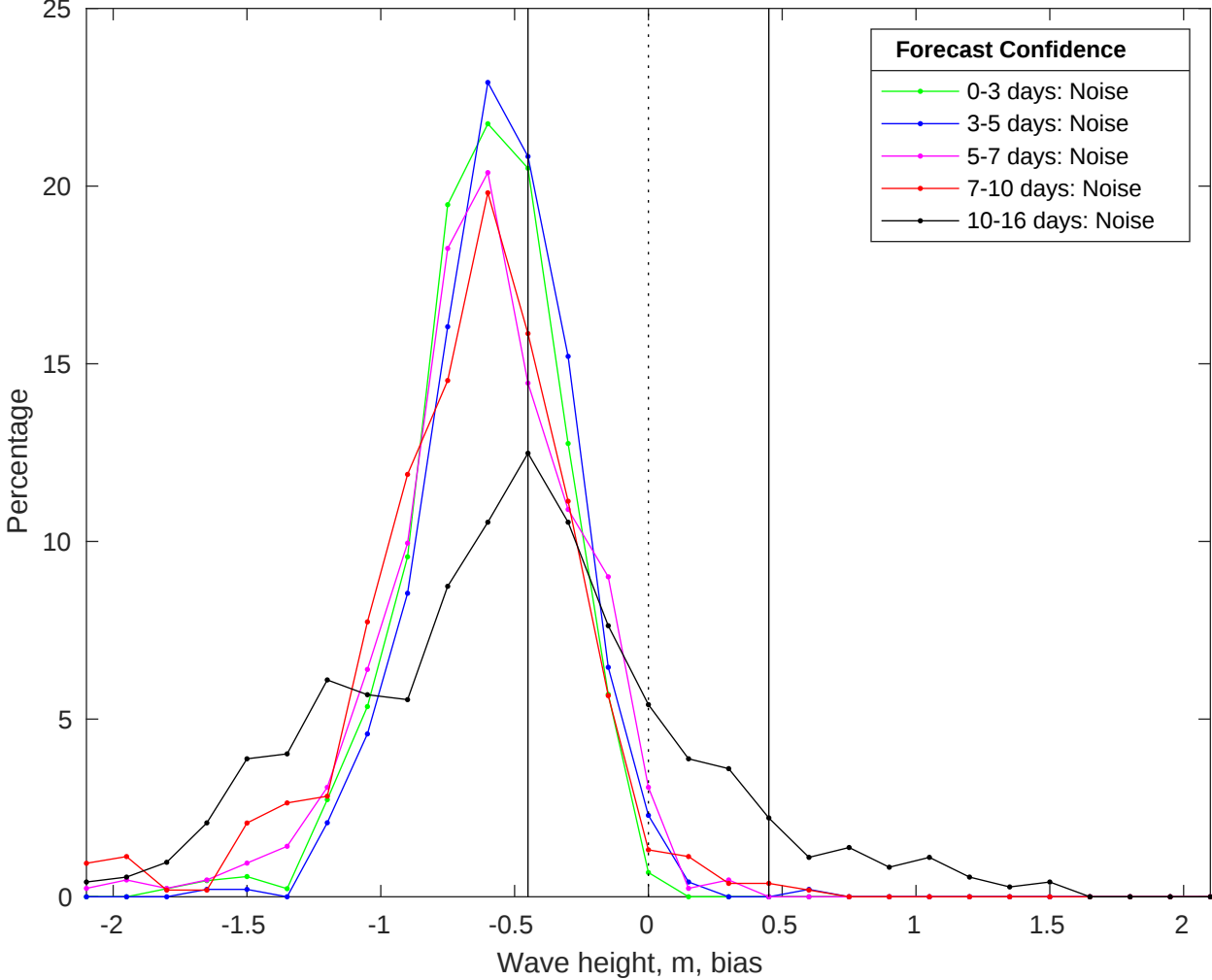
NDBC 46054 vs GFSWaves Bias Histogram: 20-Jan-2025
