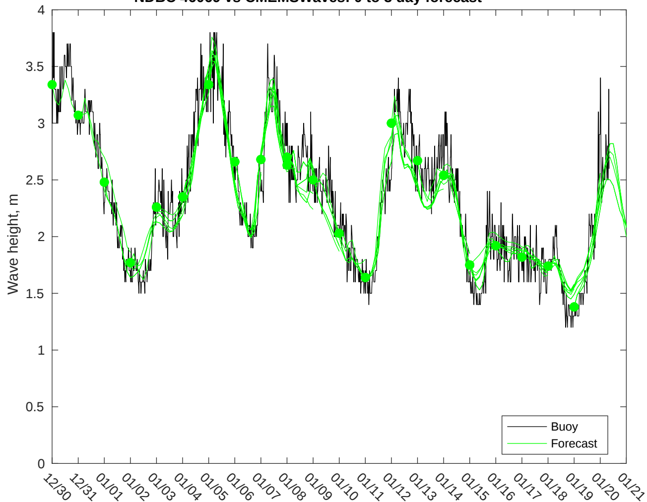
NDBC 46069 vs CMEMSWaves: 0 to 3 day forecast
