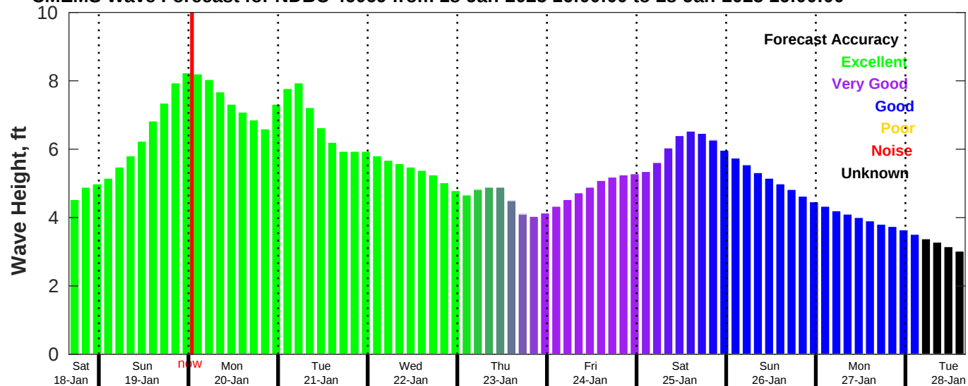
CMEMS Wave Forecast for NDBC 46069 from 18-Jan-2025 16:00:00 to 28-Jan-2025 16:00:00
