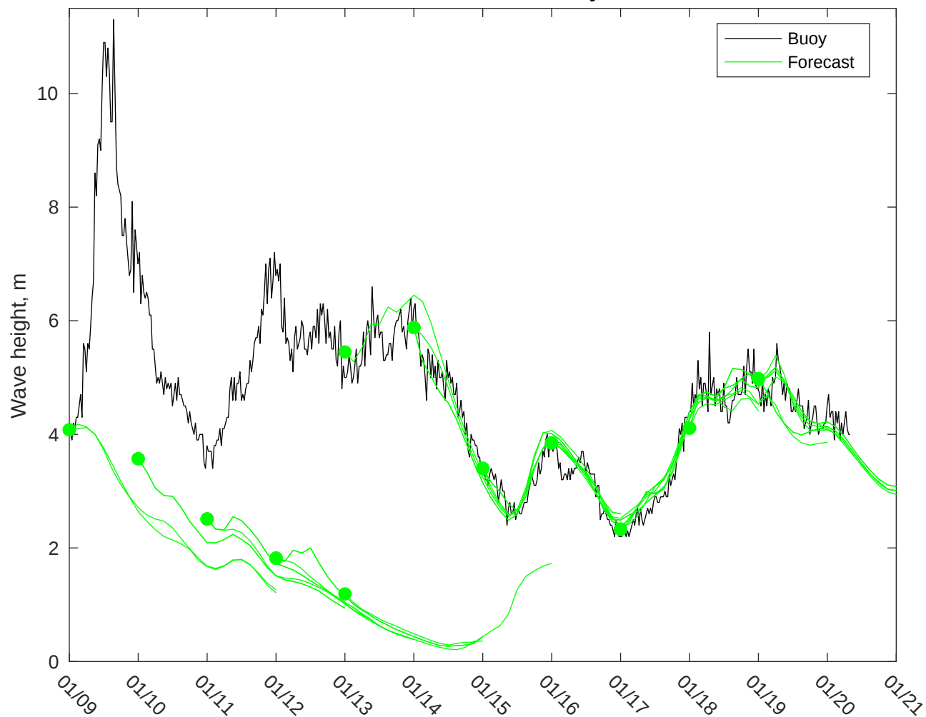
NDBC 46246 vs CMEMSWaves: 0 to 3 day forecast
