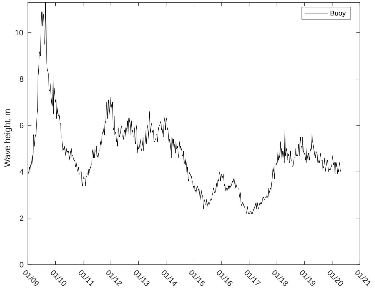
NDBC 46246 vs CMEMSWaves: 10 to 16 day forecast
