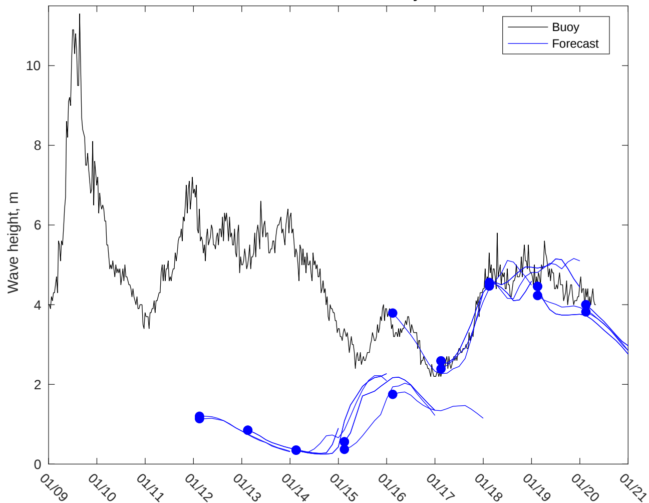
NDBC 46246 vs CMEMSWaves: 3 to 5 day forecast
