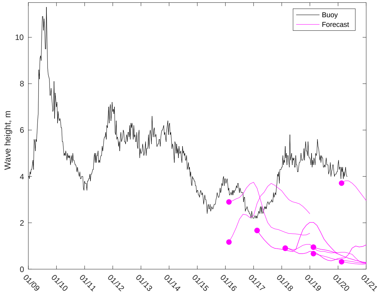
NDBC 46246 vs CMEMSWaves: 7 to 10 day forecast
