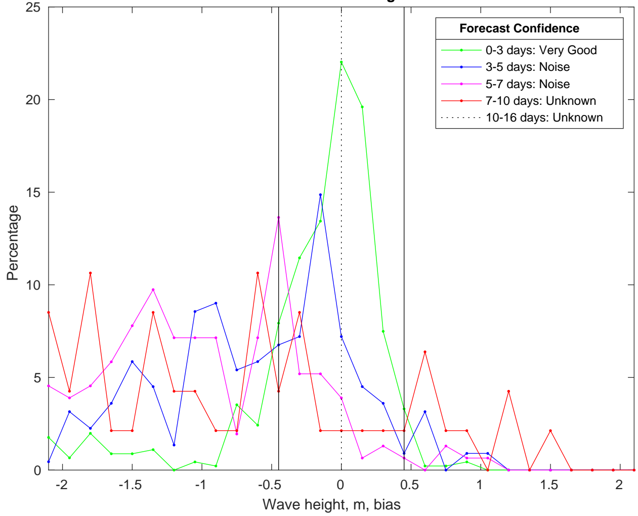
NDBC 46246 vs CMEMSWaves Bias Histogram: 20-Jan-2025
