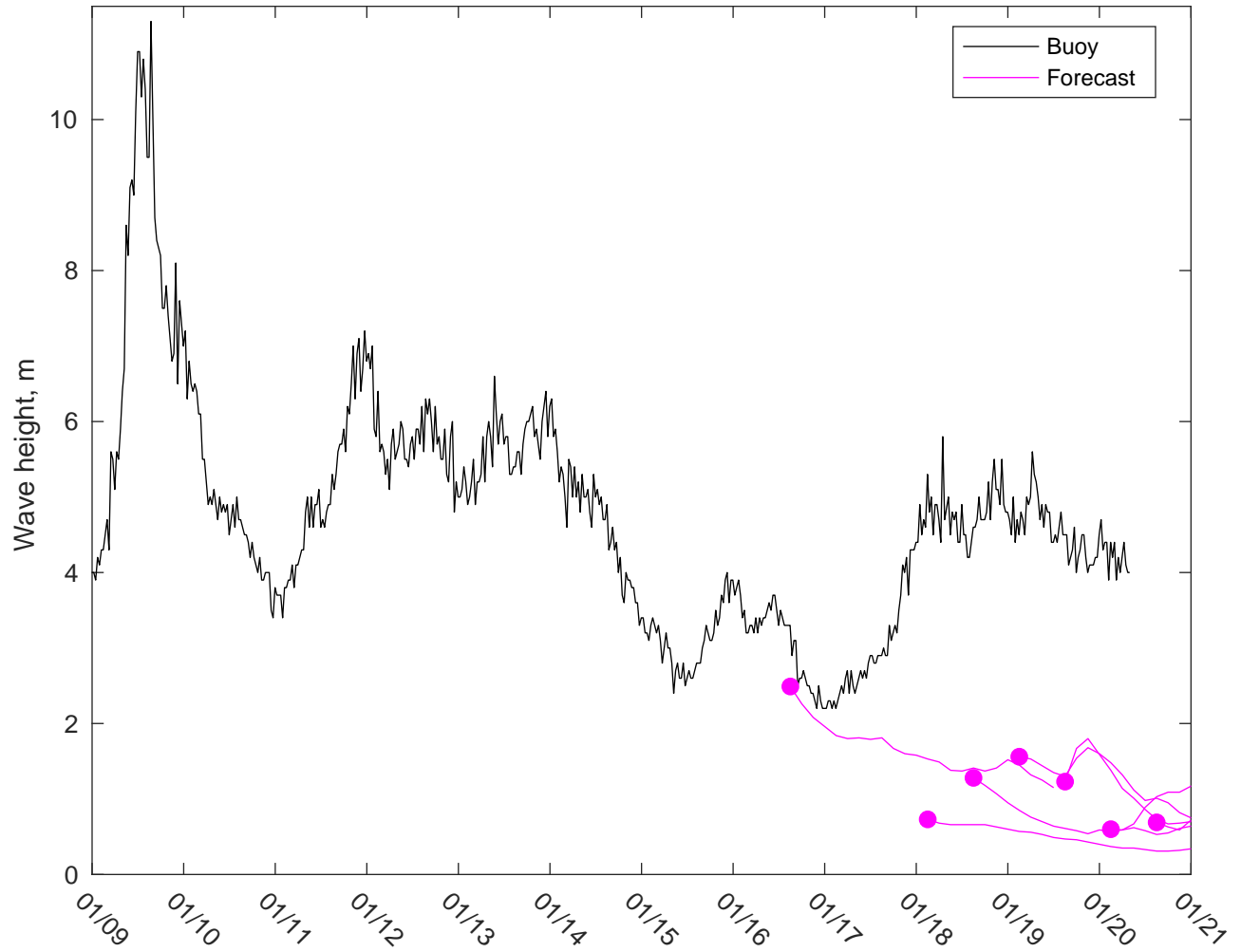
NDBC 46246 vs GFSWaves: 7 to 10 day forecast
