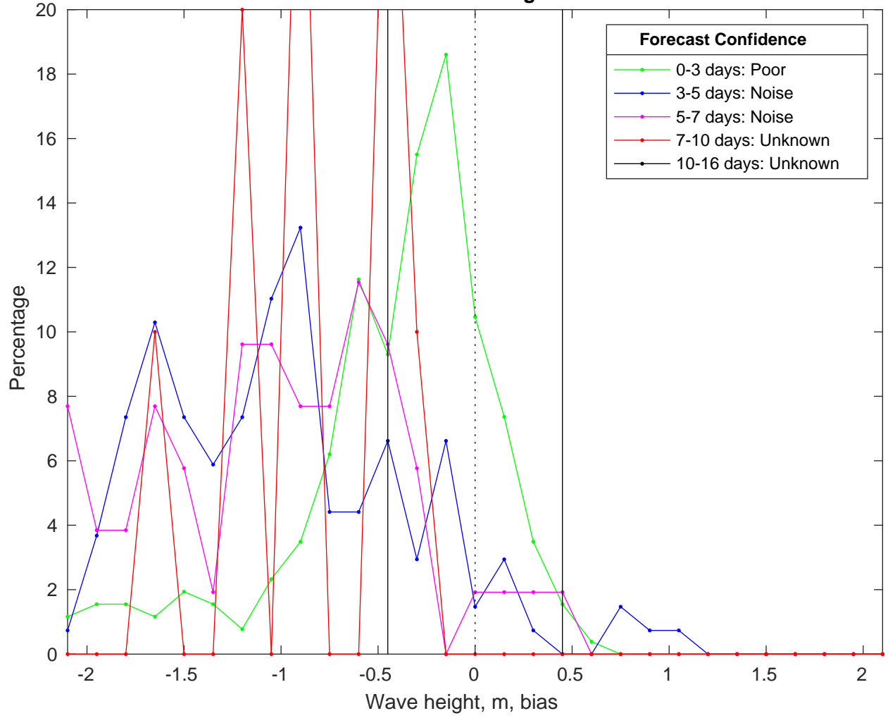
NDBC 46246 vs GFSWaves Bias Histogram: 20-Jan-2025
