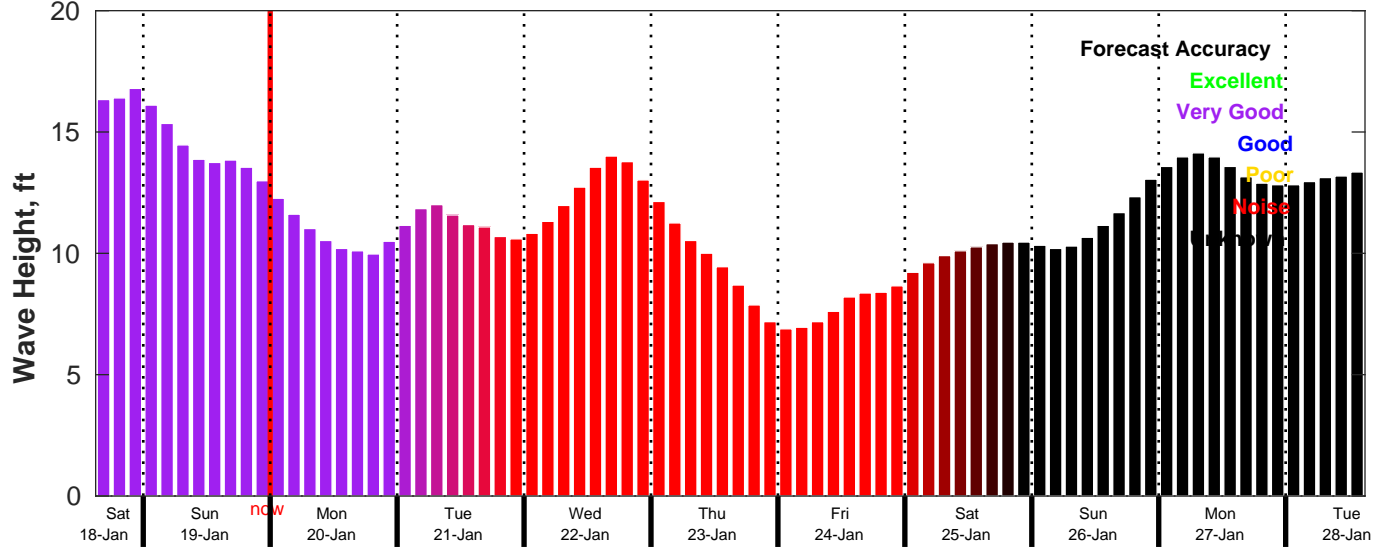
CMEMS Wave Forecast for NDBC 46246 from 18-Jan-2025 15:00:00 to 28-Jan-2025 15:00:00
