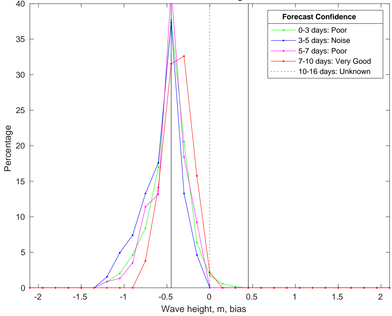
NDBC 51209 vs CMEMSWaves Bias Histogram: 20-Jan-2025
