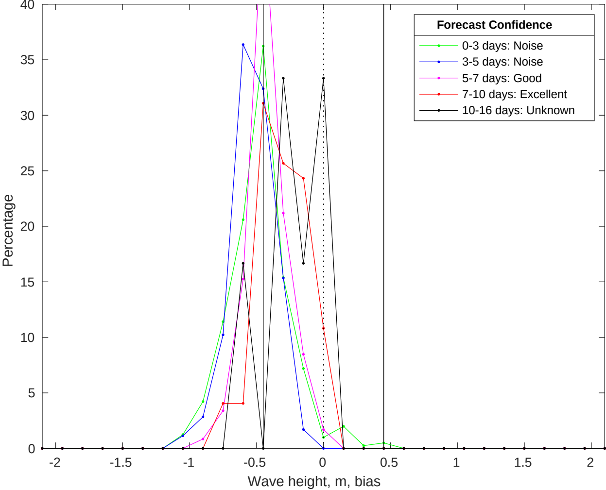
NDBC 51209 vs GFSWaves Bias Histogram: 20-Jan-2025
