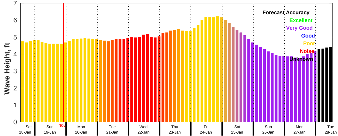
CMEMS Wave Forecast for NDBC 51209 from 18-Jan-2025 13:00:00 to 28-Jan-2025 13:00:00
