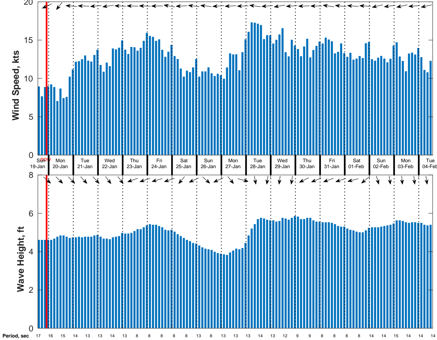
Wind & Wave Forecast for NDBC 51209 from 19-Jan-2025 13:00:00 to 04-Feb-2025 13:00:00
