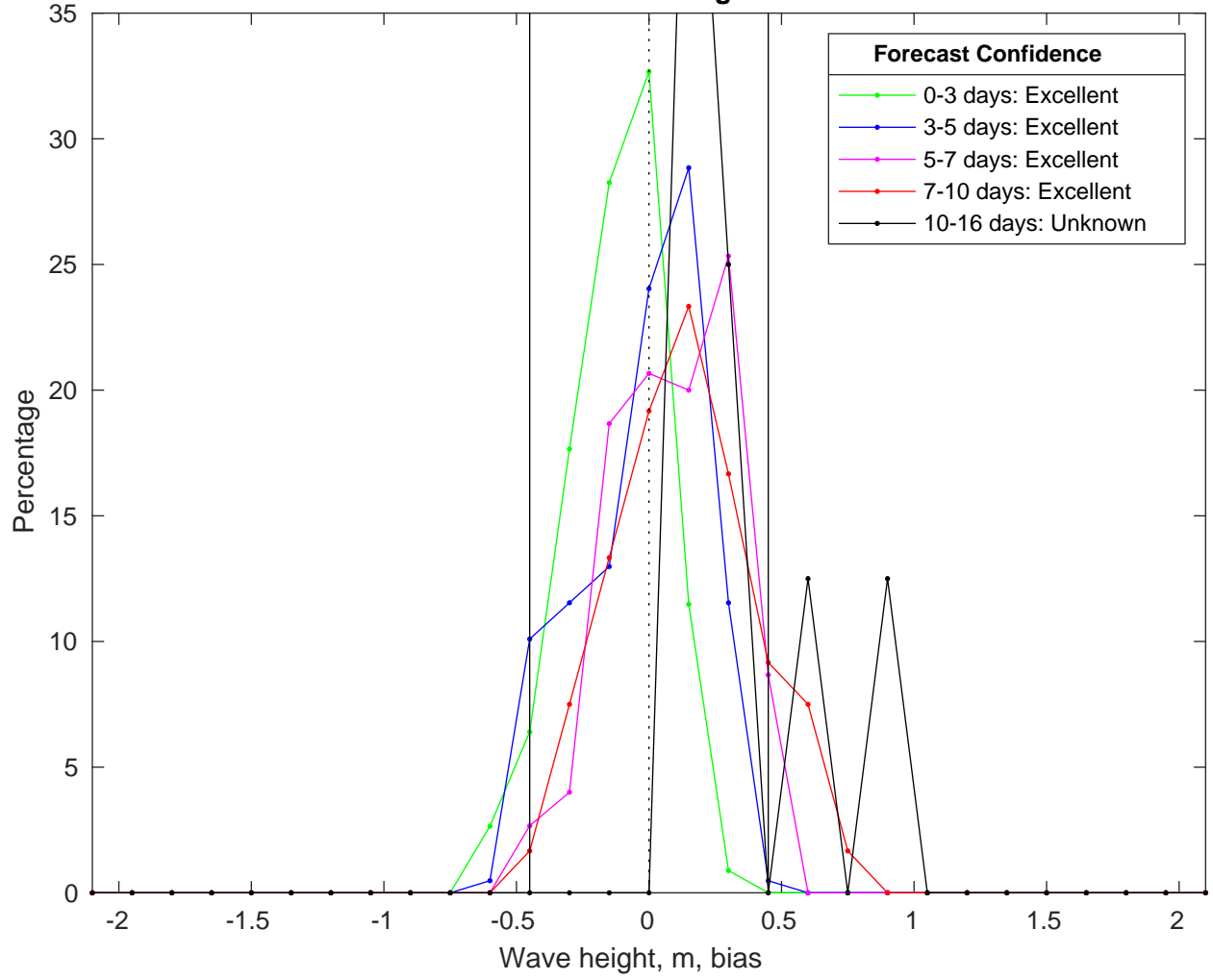
NDBC 52211 vs GFSWaves Bias Histogram: 20-Jan-2025
