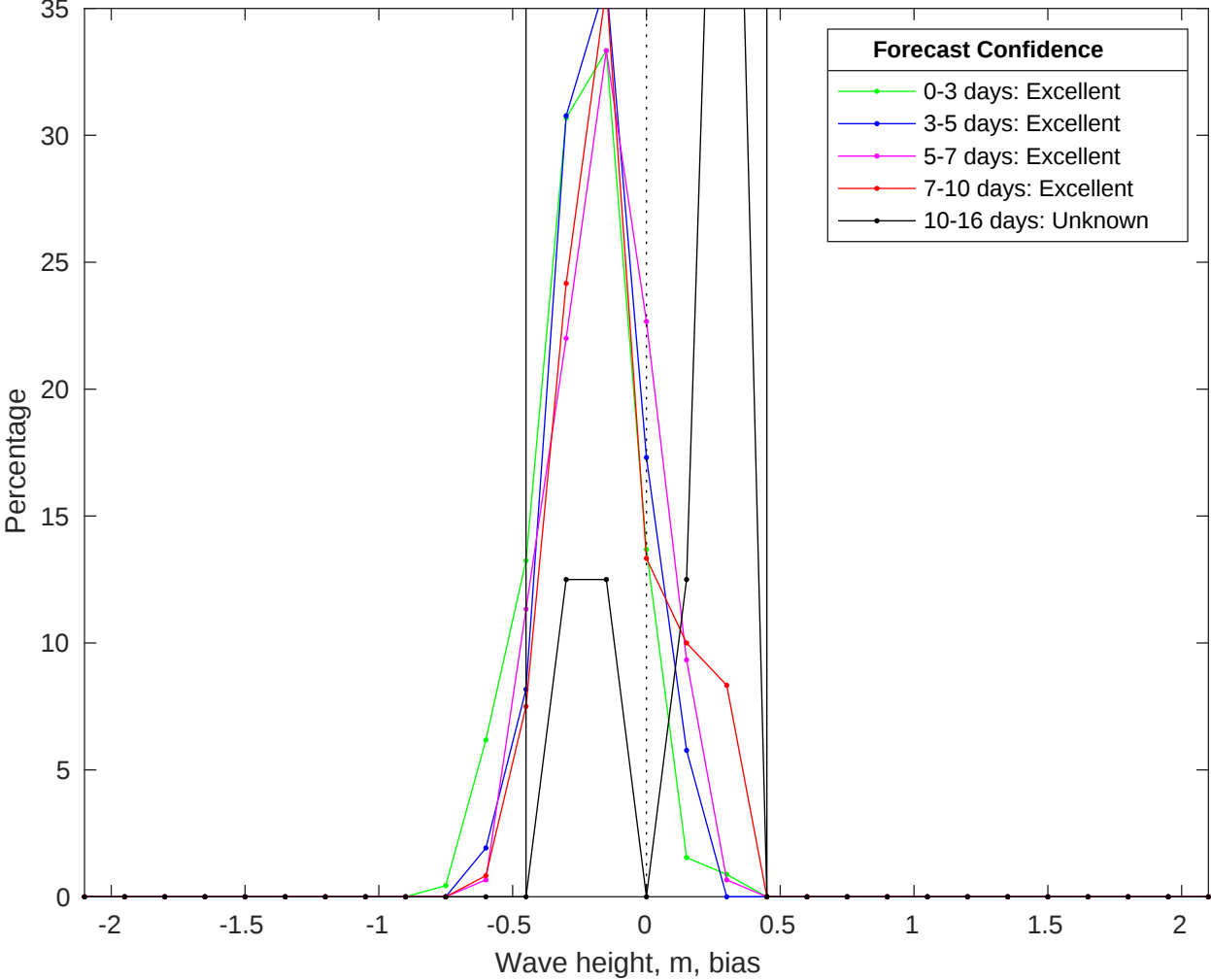
NDBC 52212 vs GFSWaves Bias Histogram: 20-Jan-2025
