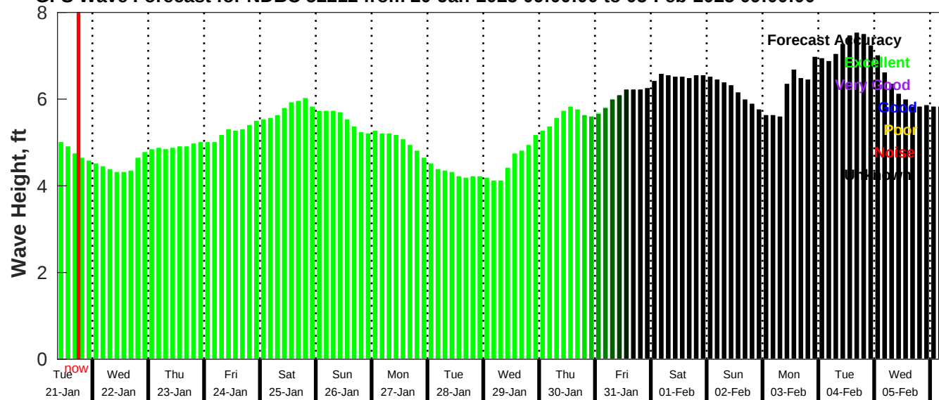
GFS Wave Forecast for NDBC 52212 from 20-Jan-2025 09:00:00 to 05-Feb-2025 09:00:00
