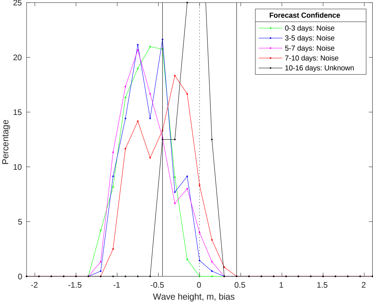
NDBC 52213 vs GFSWaves Bias Histogram: 20-Jan-2025
