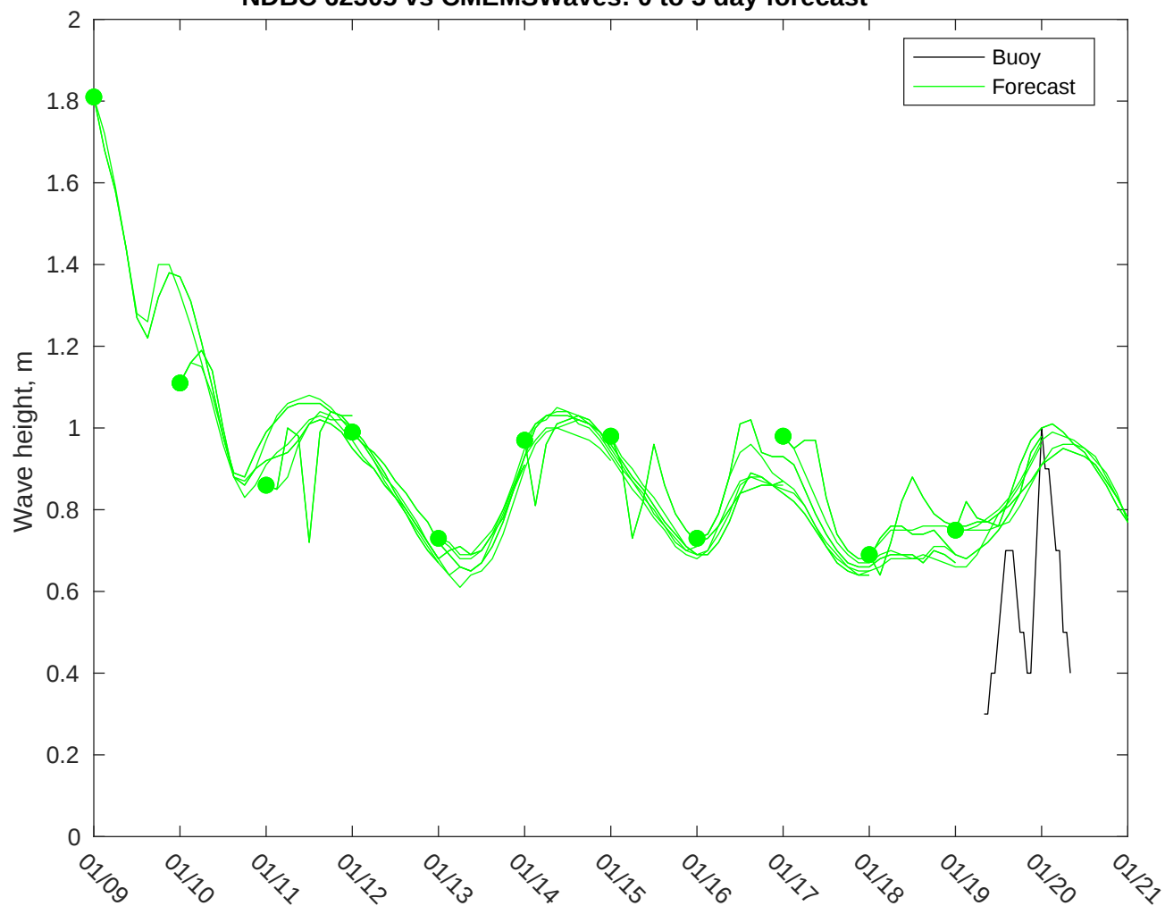
NDBC 62305 vs CMEMSWaves: 0 to 3 day forecast
