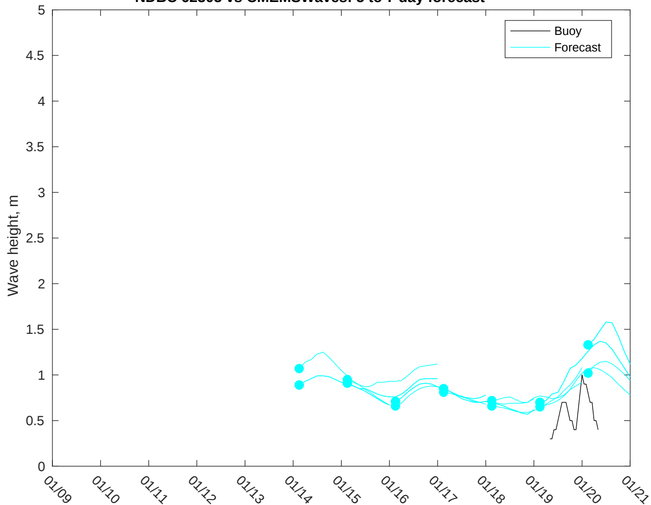
NDBC 62305 vs CMEMSWaves: 5 to 7 day forecast
