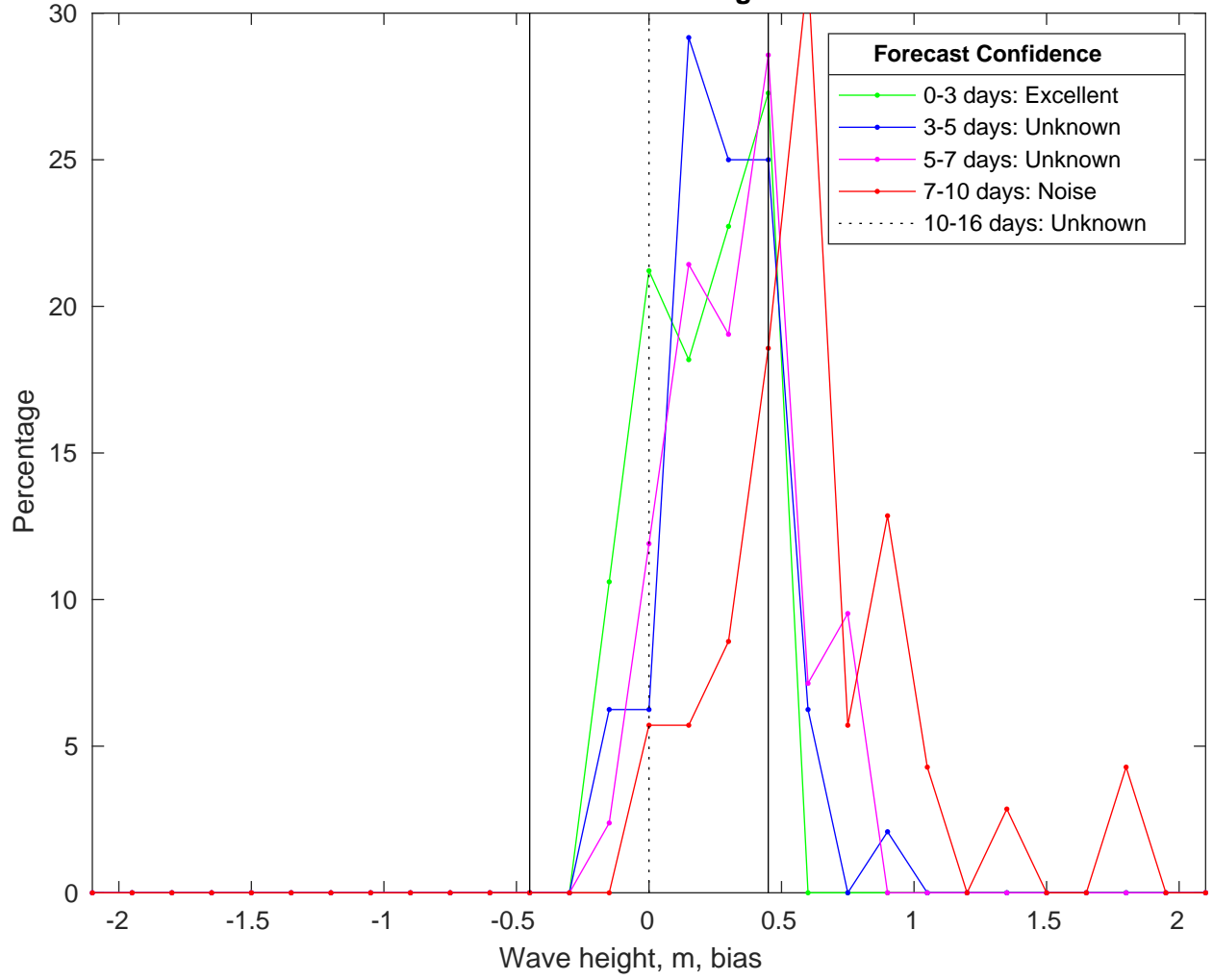
NDBC 62305 vs CMEMSWaves Bias Histogram: 20-Jan-2025
