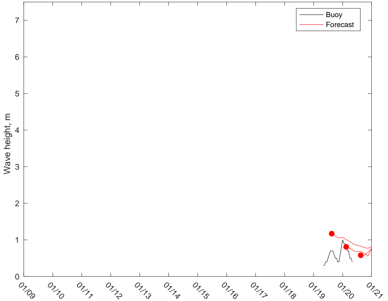
NDBC 62305 vs GFSWaves: 10 to 16 day forecast
