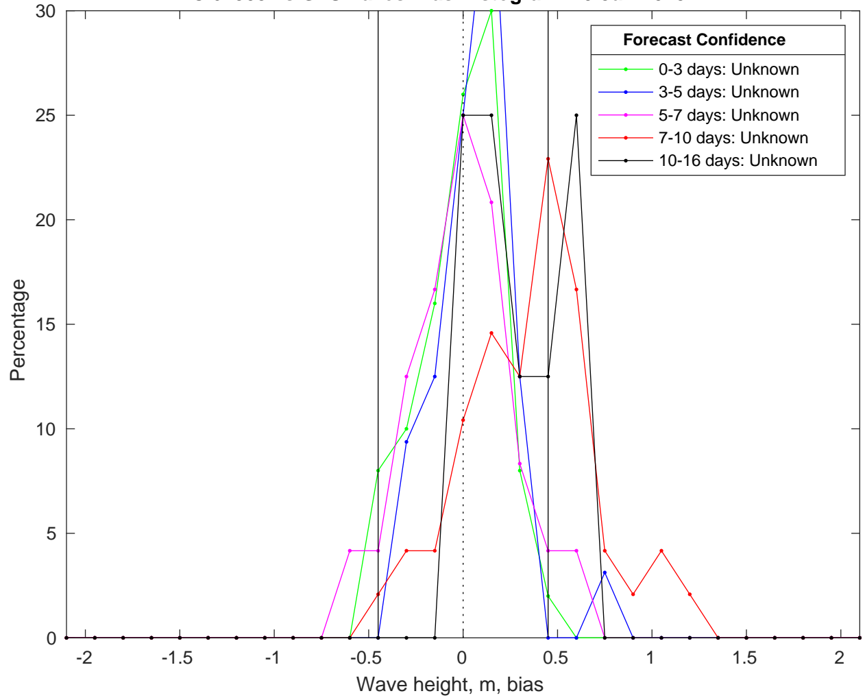
NDBC 62305 vs GFSWaves Bias Histogram: 20-Jan-2025
