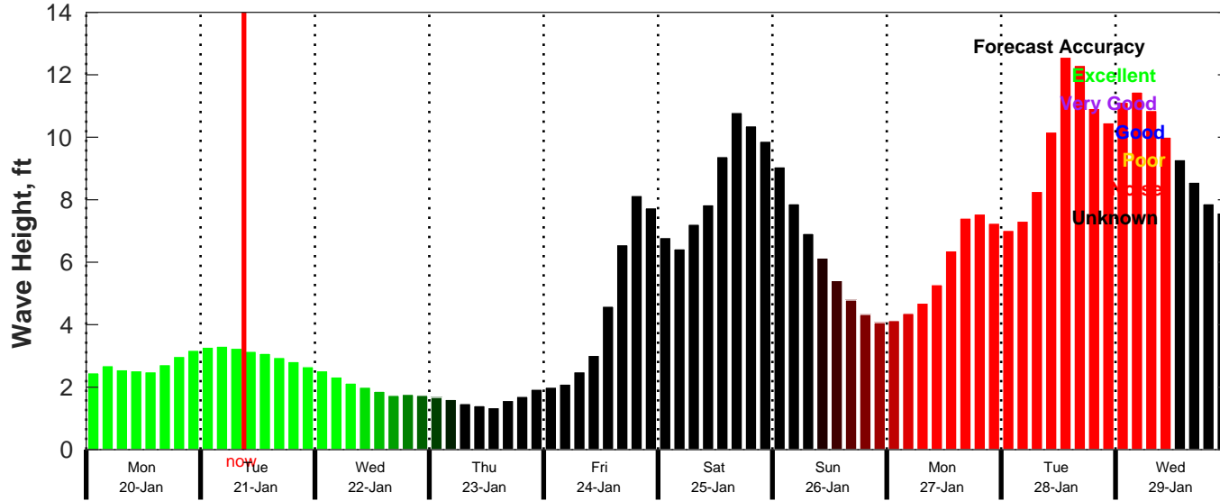
CMEMS Wave Forecast for NDBC 62305 from 19-Jan-2025 00:00:00 to 29-Jan-2025 00:00:00
