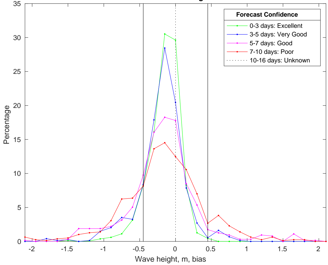
NDBC 41004 vs CMEMSWaves Bias Histogram: 21-Jan-2025
