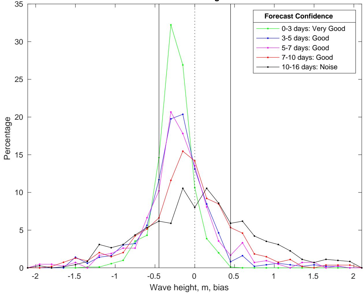
NDBC 41004 vs GFSWaves Bias Histogram: 21-Jan-2025
