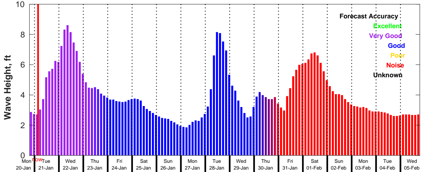
GFS Wave Forecast for NDBC 41004 from 20-Jan-2025 19:00:00 to 05-Feb-2025 19:00:00
