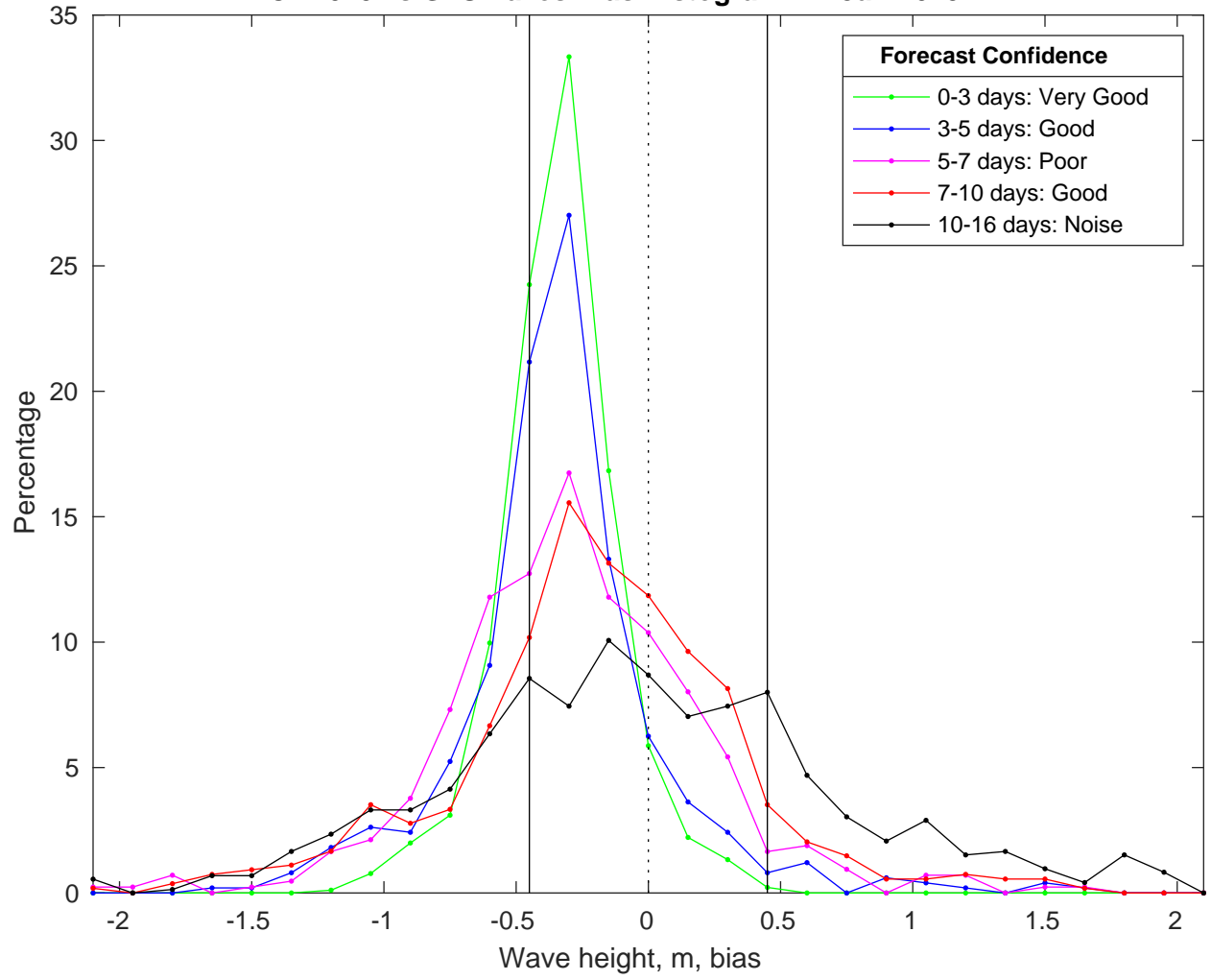
NDBC 41013 vs GFSWaves Bias Histogram: 21-Jan-2025
