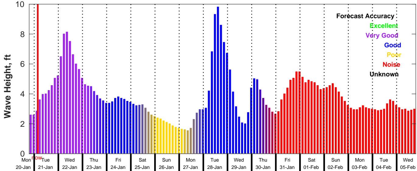
GFS Wave Forecast for NDBC 41013 from 20-Jan-2025 19:00:00 to 05-Feb-2025 19:00:00
