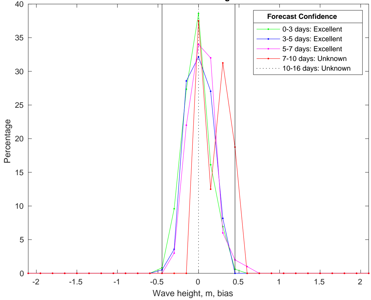
NDBC 41040 vs CMEMSWaves Bias Histogram: 21-Jan-2025
