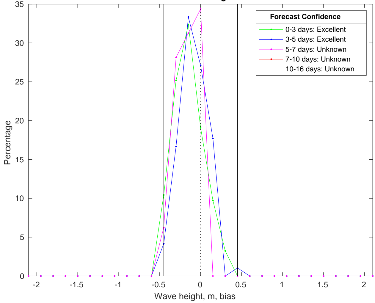
NDBC 41040 vs GFSWaves Bias Histogram: 21-Jan-2025
