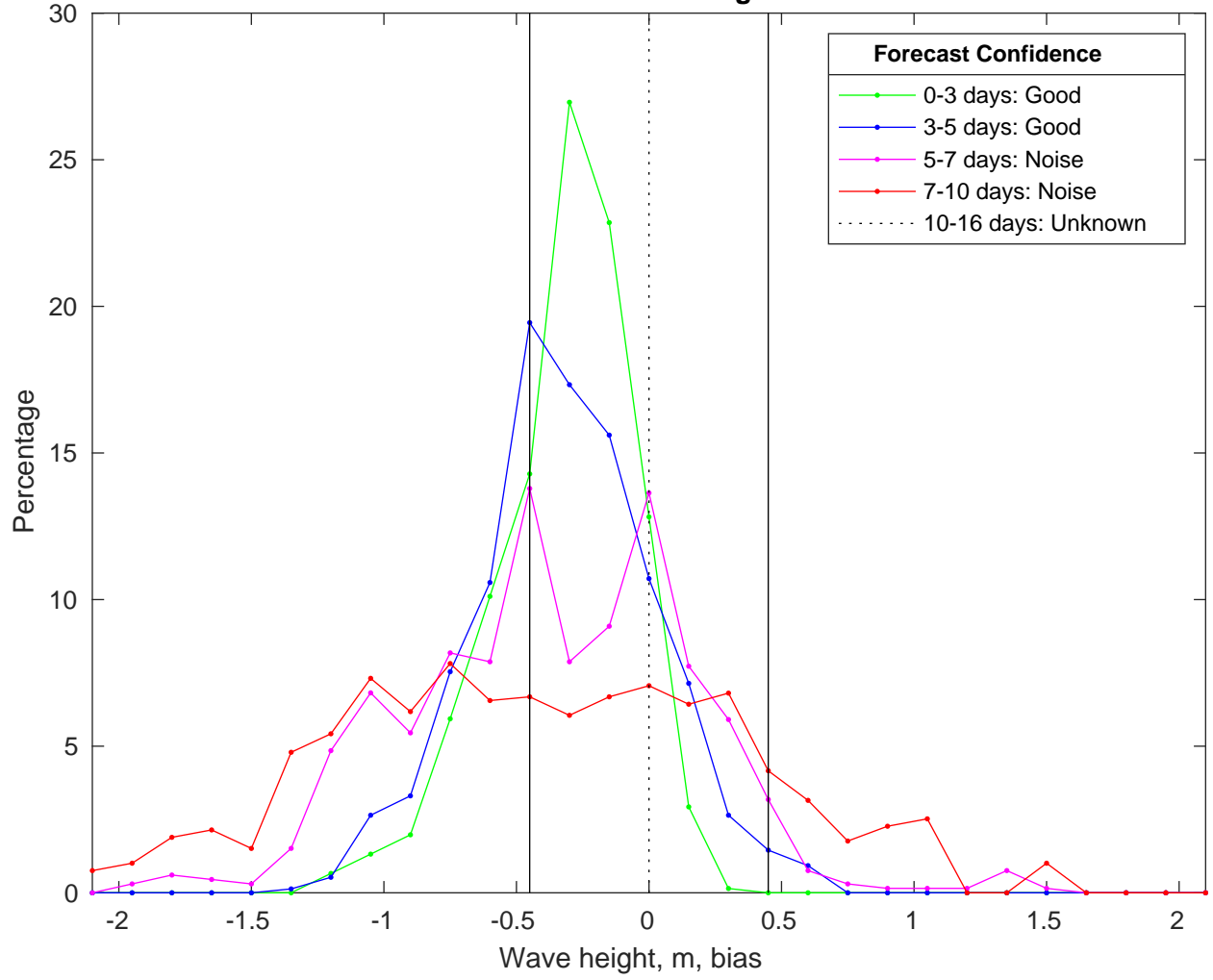
NDBC 42019 vs CMEMSWaves Bias Histogram: 21-Jan-2025
