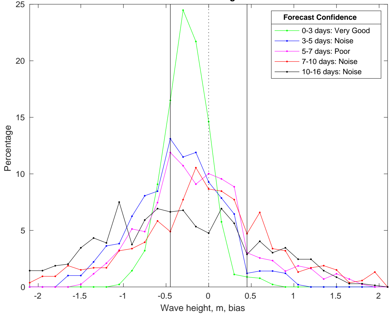
NDBC 42019 vs GFSWaves Bias Histogram: 21-Jan-2025
