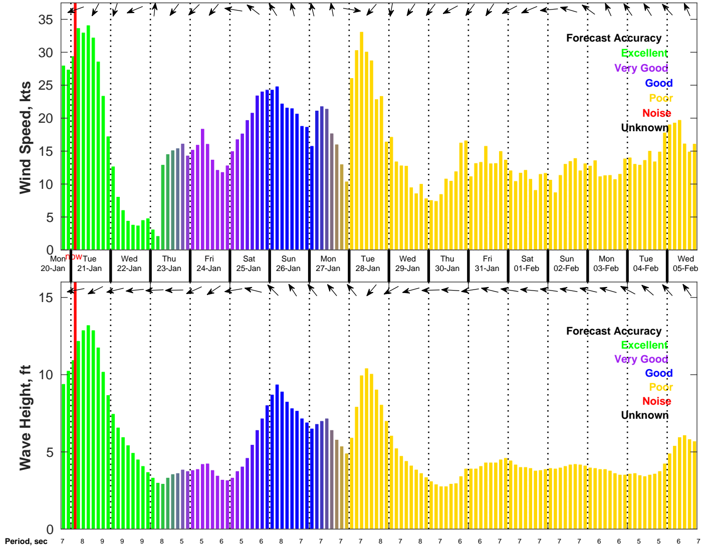
Wind & Wave Forecast for NDBC 42019 from 20-Jan-2025 18:00:00 to 05-Feb-2025 18:00:00
