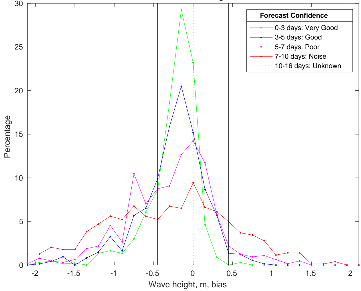
NDBC 42020 vs CMEMSWaves Bias Histogram: 21-Jan-2025
