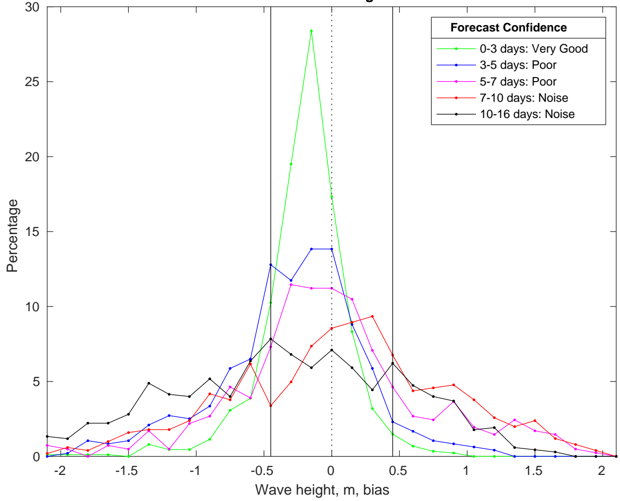
NDBC 42020 vs GFSWaves Bias Histogram: 21-Jan-2025
