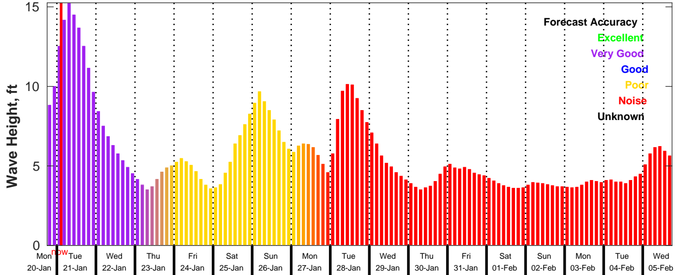
GFS Wave Forecast for NDBC 42020 from 20-Jan-2025 18:00:00 to 05-Feb-2025 18:00:00
