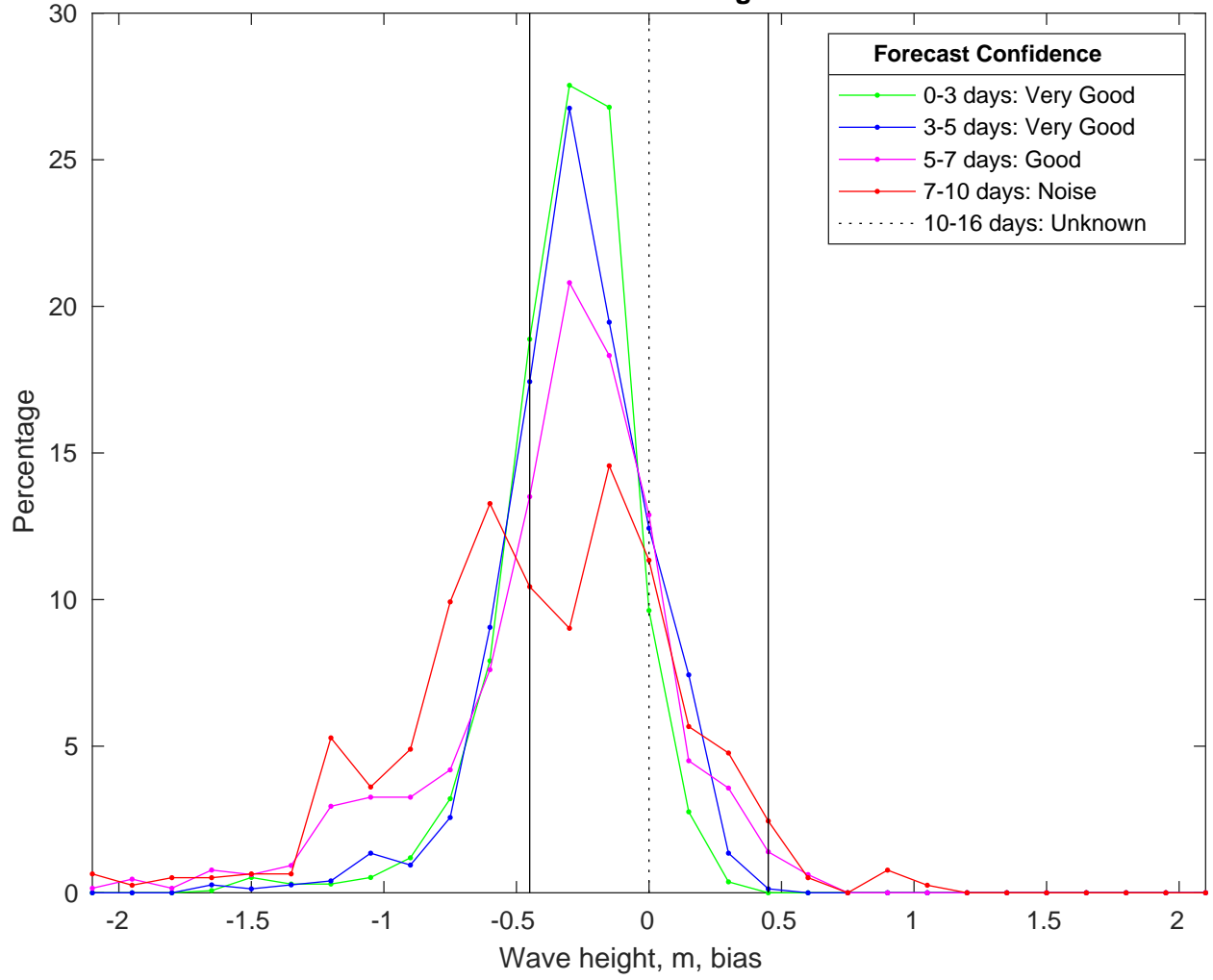
NDBC 42035 vs CMEMSWaves Bias Histogram: 21-Jan-2025
