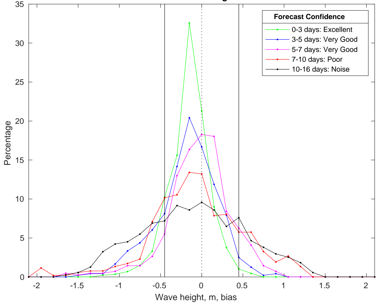
NDBC 42035 vs GFSWaves Bias Histogram: 21-Jan-2025
