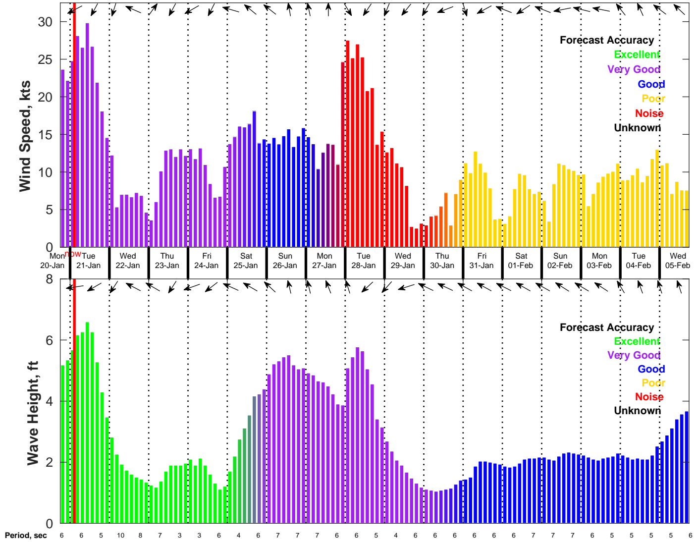
Wind & Wave Forecast for NDBC 42035 from 20-Jan-2025 18:00:00 to 05-Feb-2025 18:00:00
