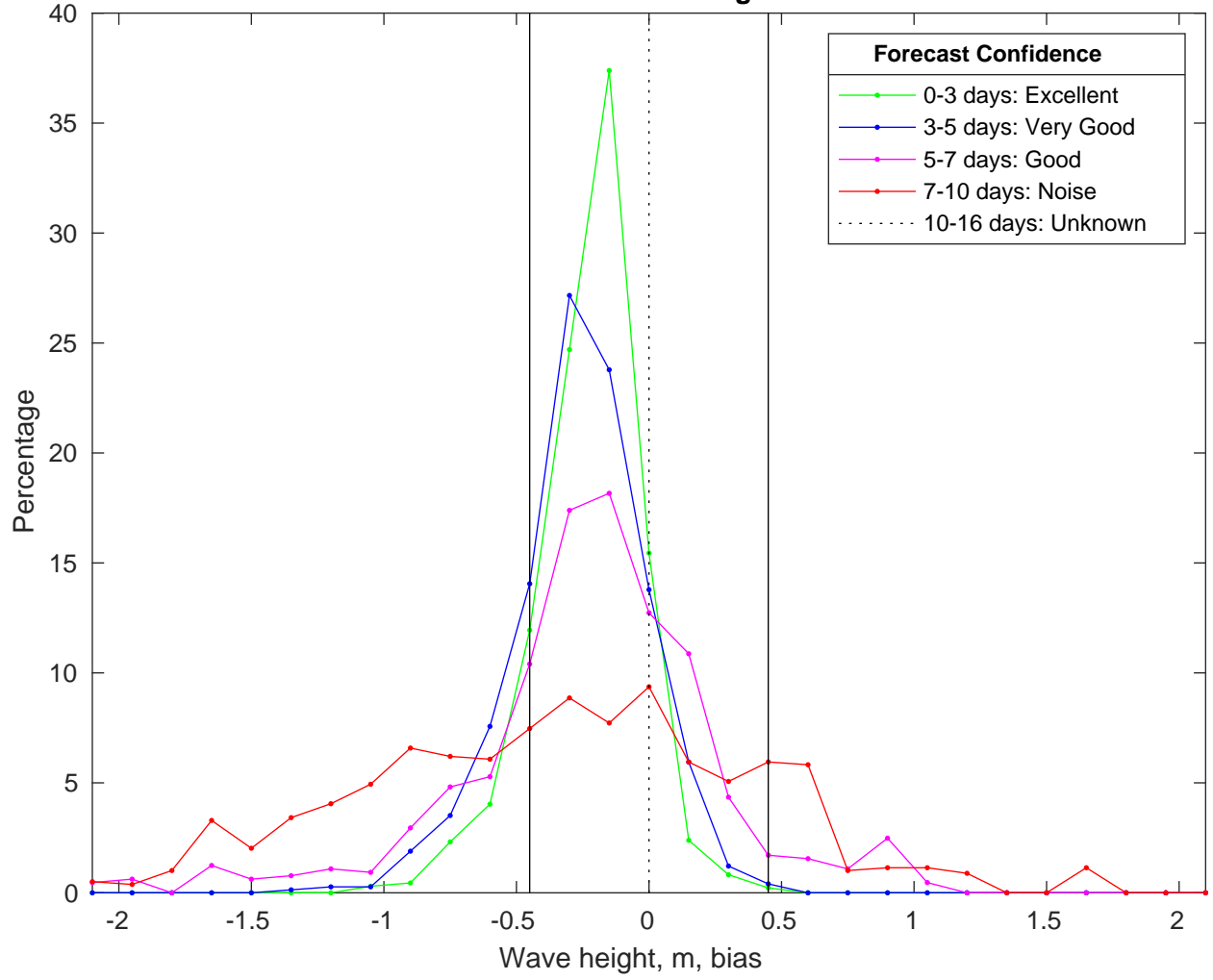
NDBC 42036 vs CMEMSWaves Bias Histogram: 21-Jan-2025
