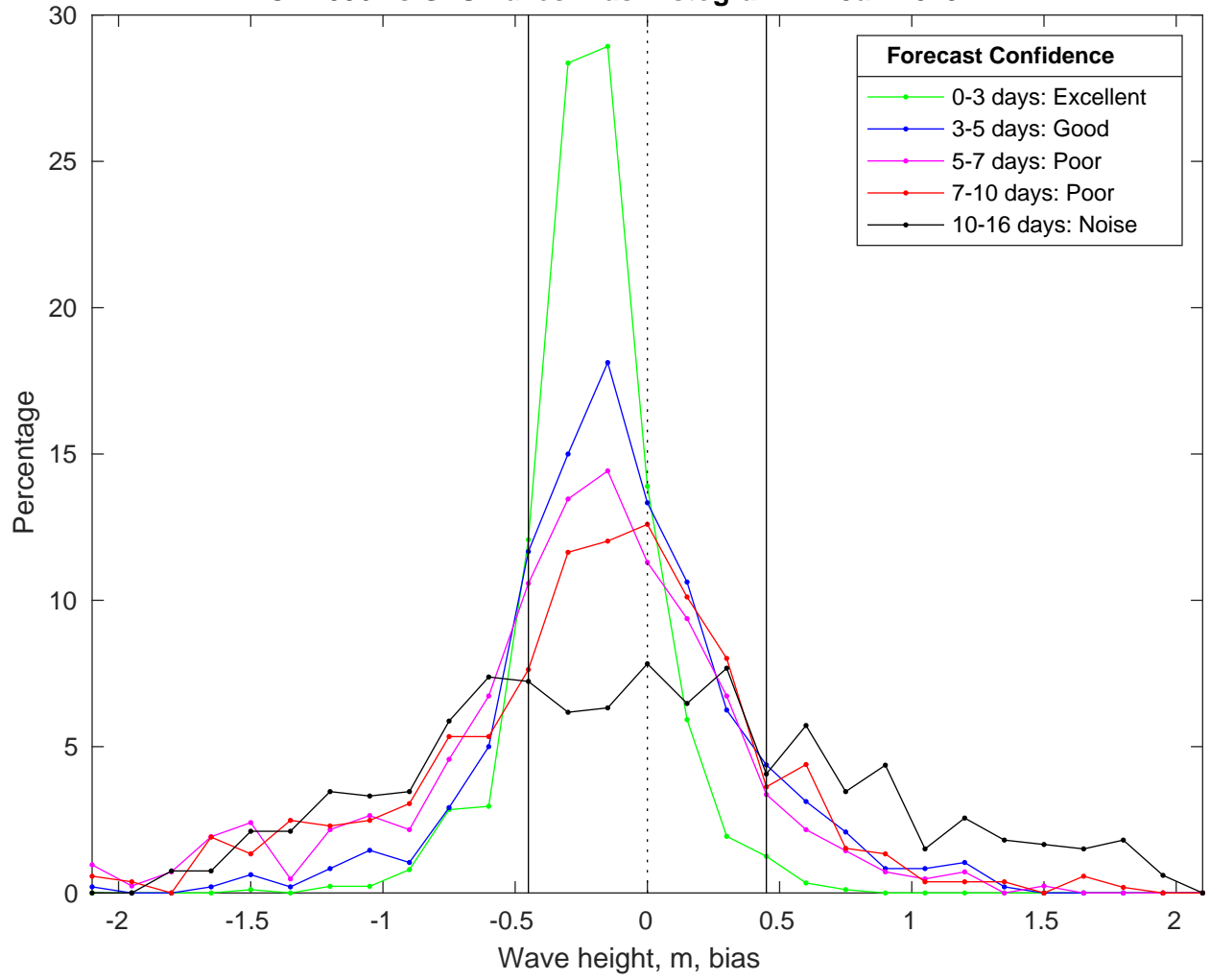
NDBC 42036 vs GFSWaves Bias Histogram: 21-Jan-2025
