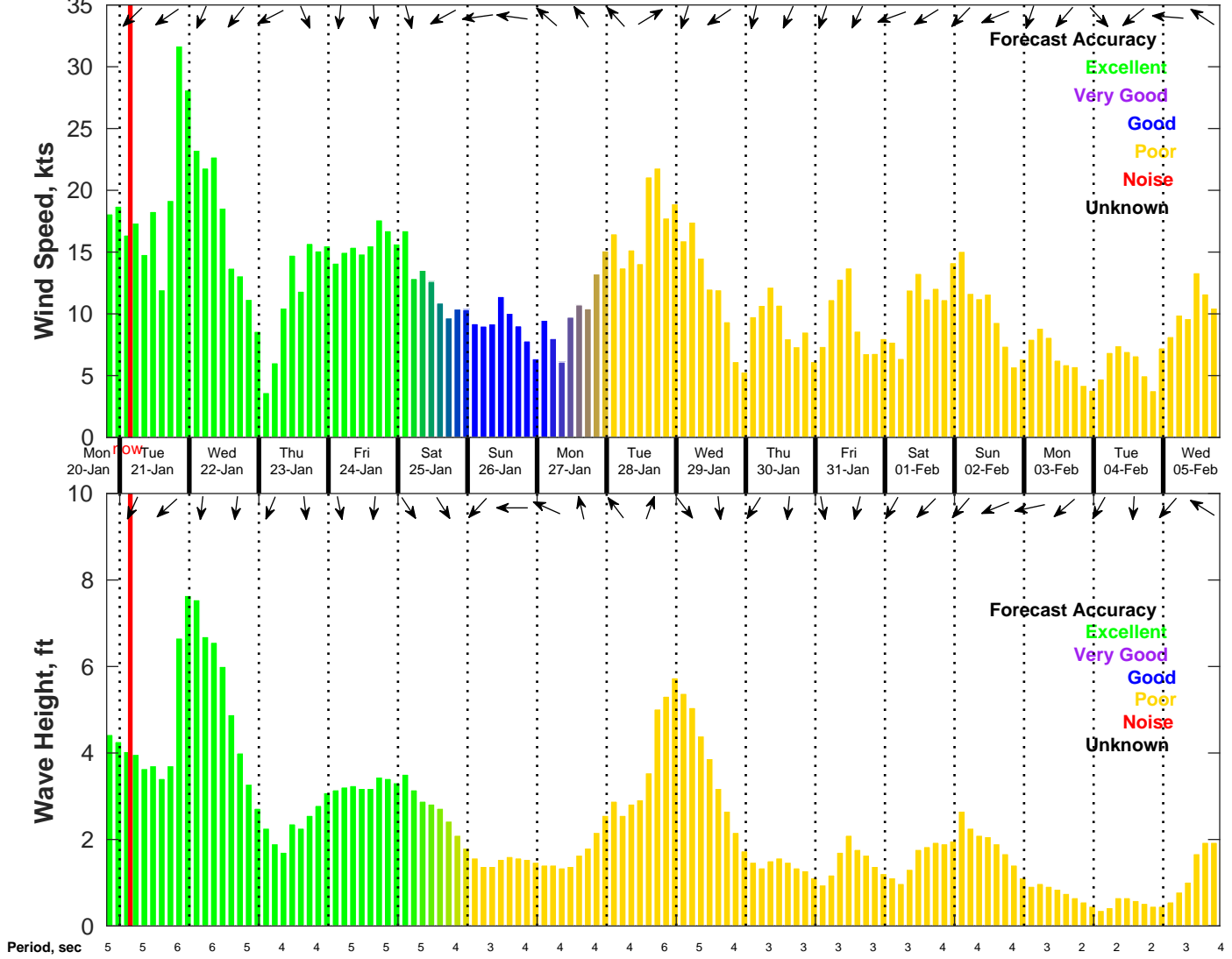
Wind & Wave Forecast for NDBC 42036 from 20-Jan-2025 19:00:00 to 05-Feb-2025 19:00:00
